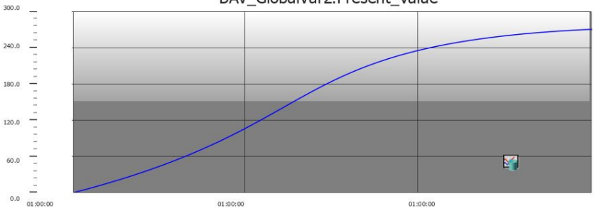
BAV_GlobalVar2.Present_Value
