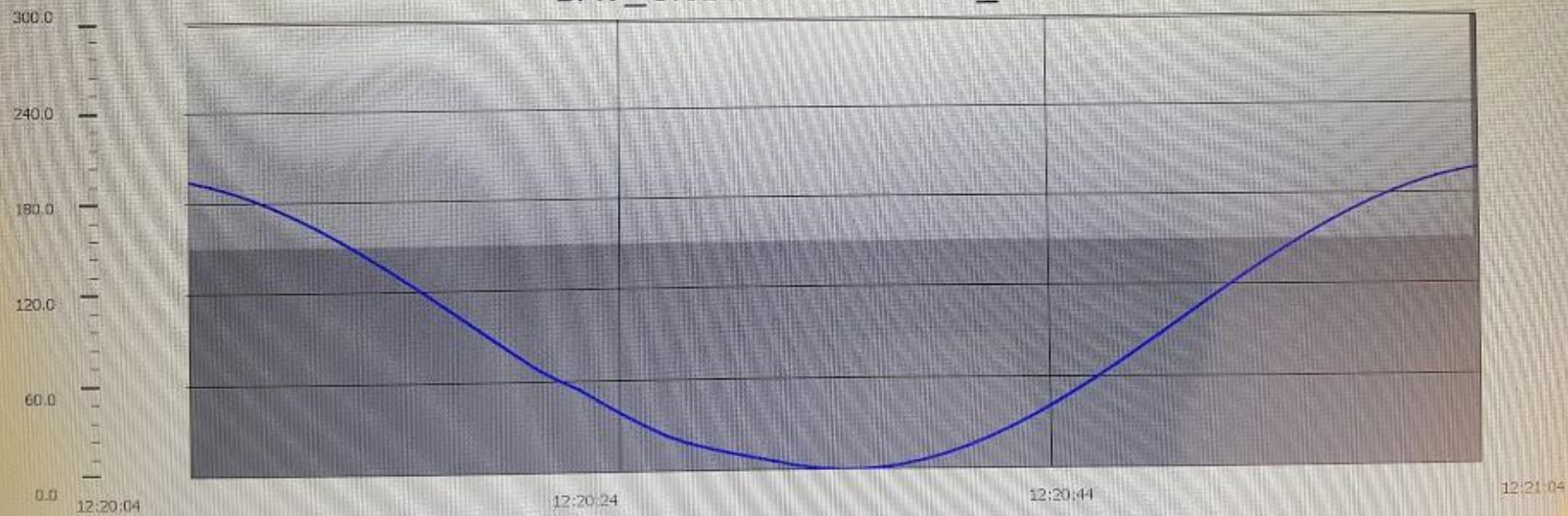
BAV_GlobalVar2.Present_Value
